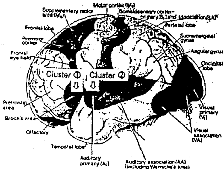
Figure 13-2 Major functional areas of cortex. (From Pandya D N, Vetterlin E H: Architecture and connections of cortical association areas. In Cerebral Cortex, vol 4, p 3. A Peters, E G Jones, editors. Plenum. New York, 1985, with permission.)
